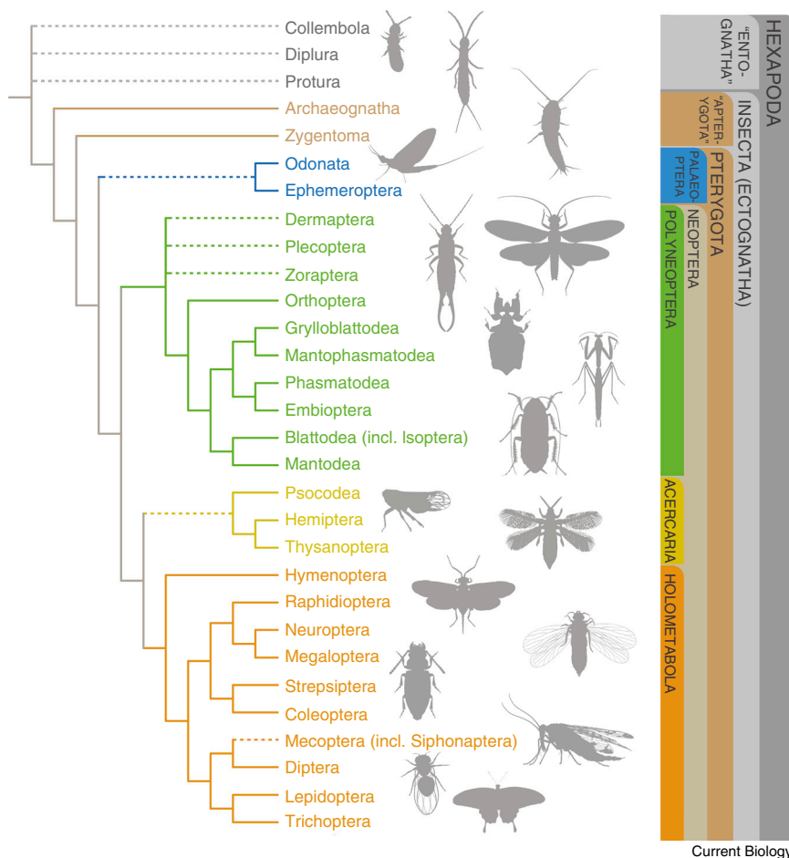
Figure 1. Insect phylogeny.
